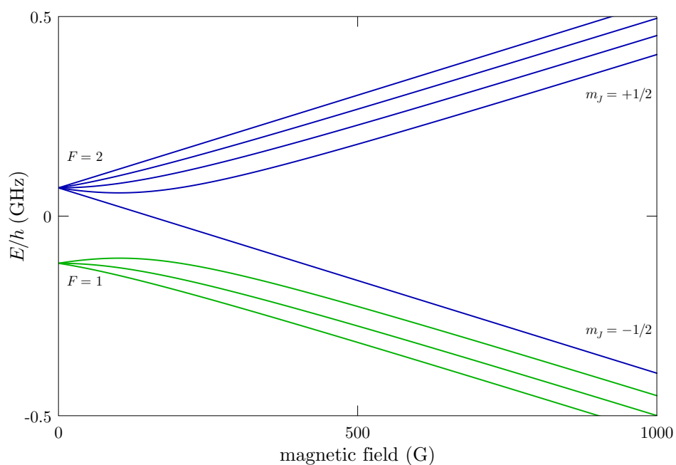
Figure 5: Sodium 3^2P_{1/2} ( D_1 excited) level hyperfine structure in an external magnetic field. The levels are grouped according to the value of F in the low-field (Zeeman) regime and m_j in the strong-field (hyperfine Paschen-Back) regime.
