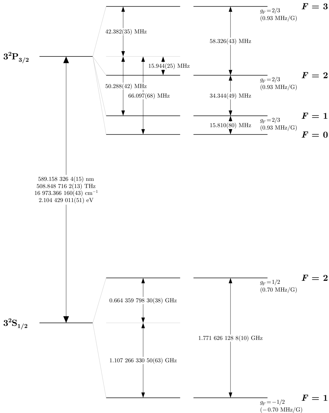
Figure 2: Sodium D 2 transition hyperfine structure, with frequency splittings between the hyperfine energy levels. The excited-state values are taken from [26], and the ground-state values are from [23]. The relative hyperfine shifts are shown to scale within each hyperfine manifold (but visual spacings should not be compared between manifolds or to the optical splitting). The approximate Landé g_F -factors for each level are also given, with the corresponding Zeeman splittings between adjacent magnetic sublevels.
