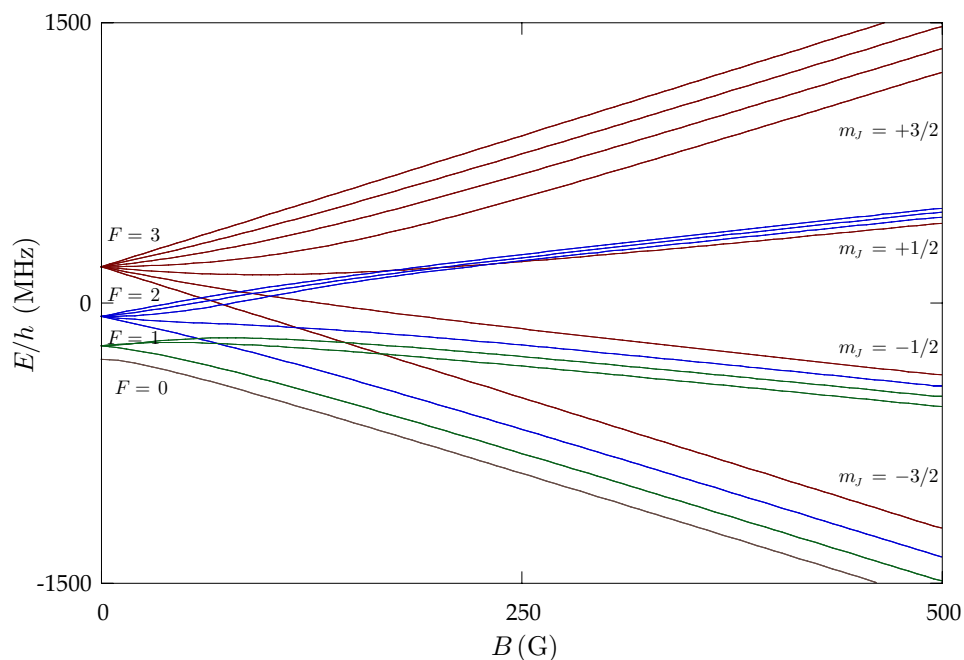
Figure 6: ^{87}\text{Rb } 5^2\text{P}_{3/2} (D 2 excited) level hyperfine structure in an external magnetic field. The levels are grouped according to the value of F in the low-field (anomalous Zeeman) regime and m_J in the strong-field (hyperfine Paschen-Back) regime.
