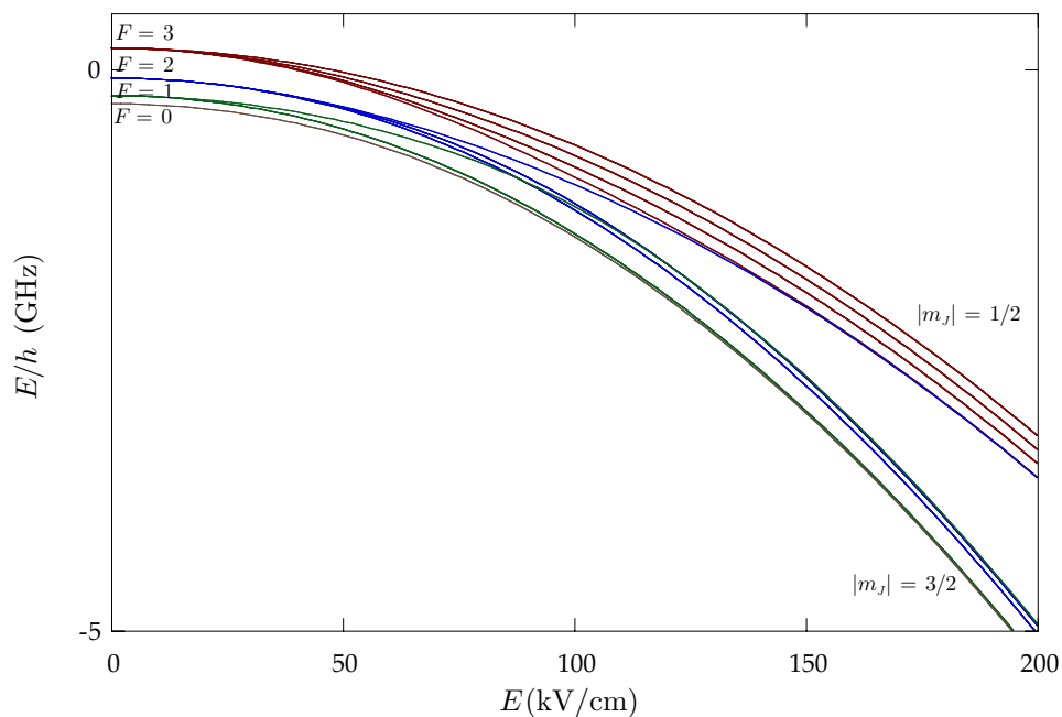
Figure 7: ^{87}\text{Rb } 5^2\text{P}_{3/2} (D 2 excited) level hyperfine structure in a constant, external electric field. The levels are grouped according to the value of F in the low-field (anomalous Zeeman) regime and |m_J| in the strong-field (“electric” hyperfine Paschen-Back) regime. Levels with the same values of F and |m_F| (for a weak field) are degenerate.
