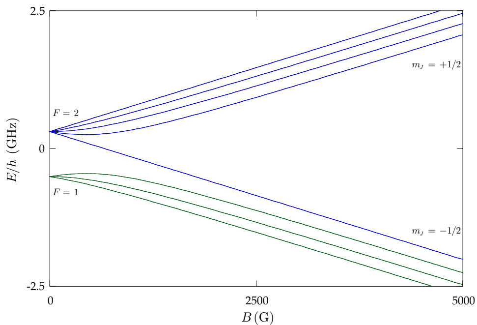
Figure 5: ^{87}\text{Rb } 5^2\text{P}_{1/2} ( D_1 excited) level hyperfine structure in an external magnetic field. The levels are grouped according to the value of F in the low-field (anomalous Zeeman) regime and m_J in the strong-field (hyperfine Paschen-Back) regime.
