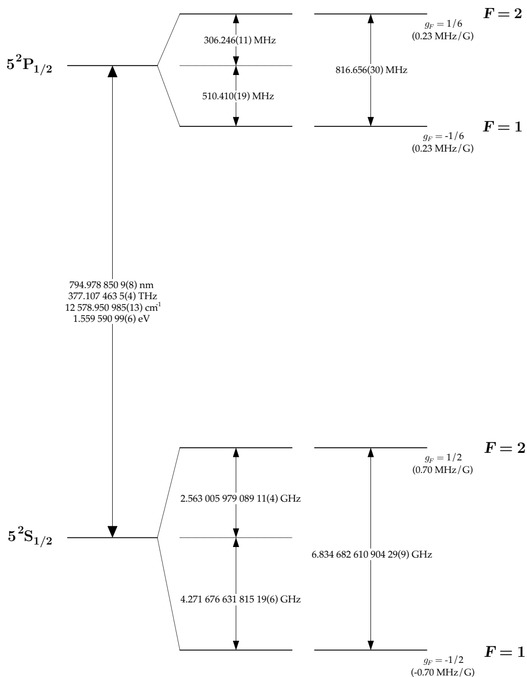
Figure 3: ^{87}\text{Rb} D_1 transition hyperfine structure, with frequency splittings between the hyperfine energy levels. The excited-state values are taken from [7], and the ground-state values are from [16]. The approximate Landé g_F -factors for each level are also given, with the corresponding Zeeman splittings between adjacent magnetic sublevels.
