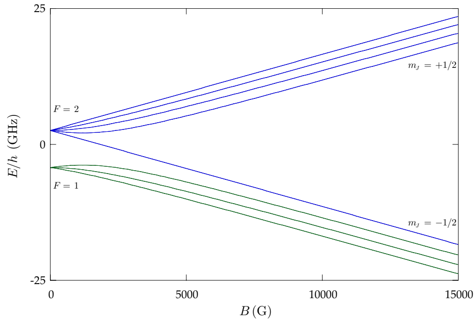
Figure 4: ^{87}\text{Rb } 5^2\text{S}_{1/2} (ground) level hyperfine structure in an external magnetic field. The levels are grouped according to the value of F in the low-field (anomalous Zeeman) regime and m_J in the strong-field (hyperfine Paschen-Back) regime.
