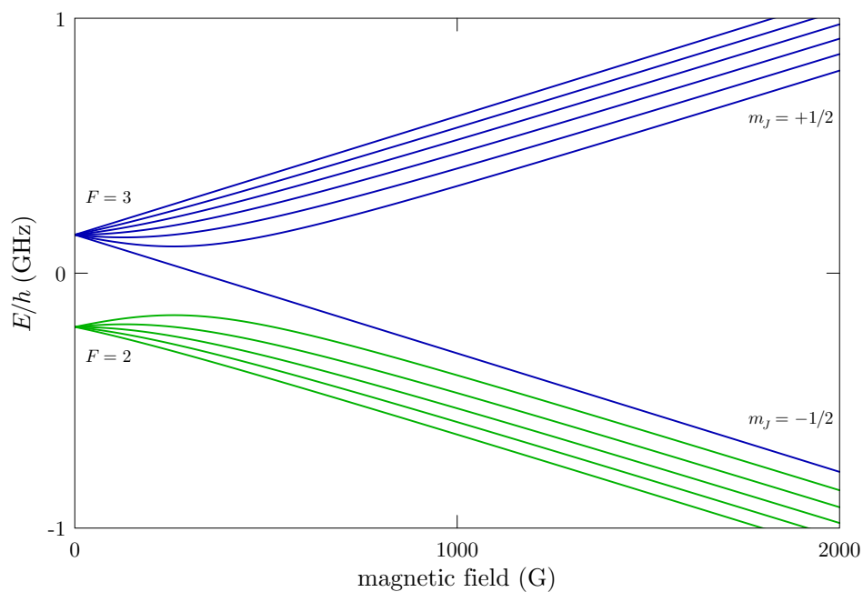
Figure 5: Rubidium 85 5^2P_{1/2} (D 1 excited) level hyperfine structure in an external magnetic field. The levels are grouped according to the value of F in the low-field (Zeeman) regime and m_J in the strong-field (hyperfine Paschen-Back) regime.
