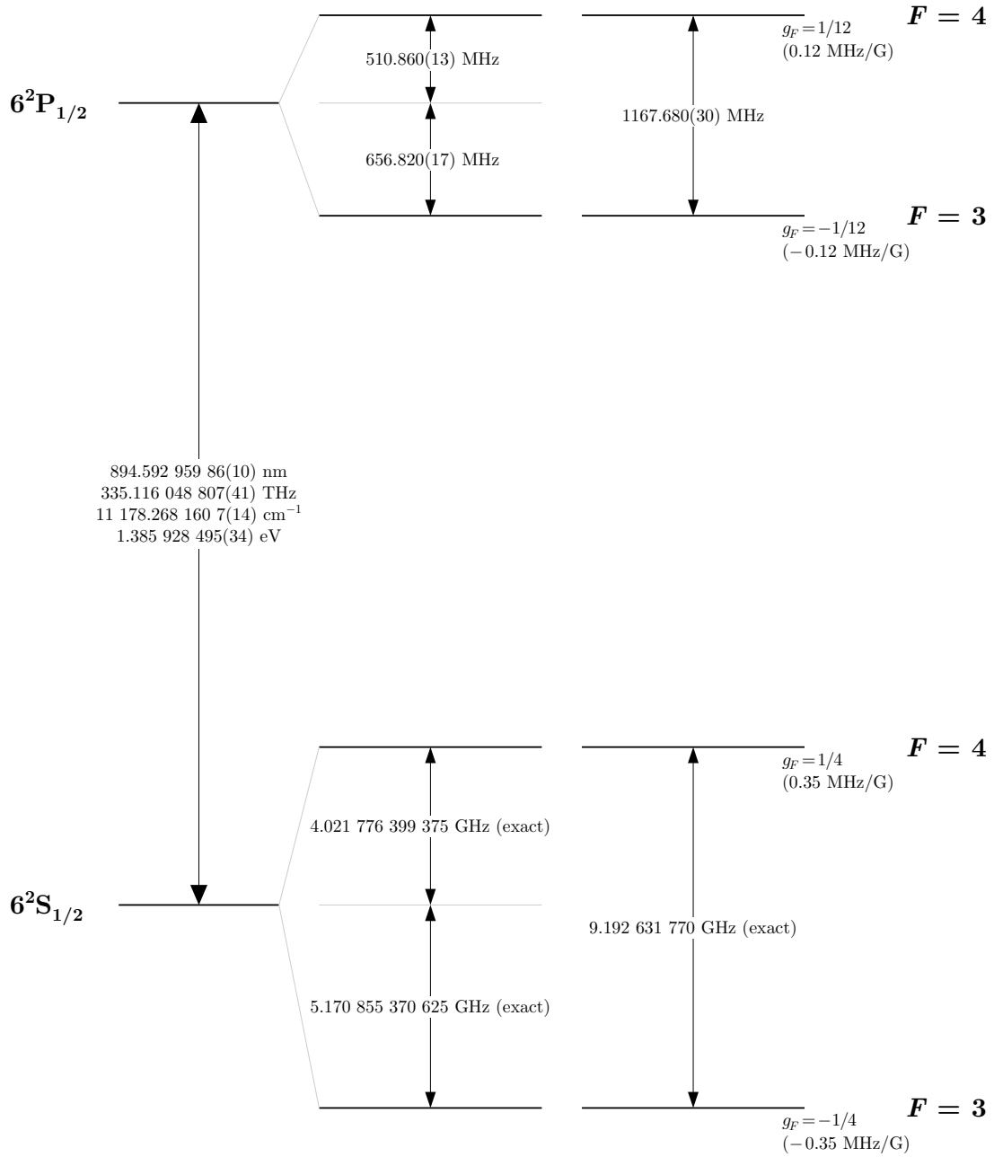
Figure 3: Cesium D_1 transition hyperfine structure, with frequency splittings between the hyperfine energy levels. The excited-state values are taken from [11, 32], and the ground-state values are exact, as a result of the current definition of the second. The relative hyperfine shifts are shown to scale within each hyperfine manifold (but visual spacings should not be compared between manifolds or to the optical splitting). The approximate Landé g_F -factors for each level are also given, with the corresponding Zeeman splittings between adjacent magnetic sublevels.
