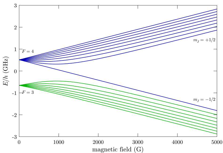
Figure 5: Cesium 6^2P_{1/2} ( D_1 excited) level hyperfine structure in an external magnetic field. The levels are grouped according to the value of F in the low-field (Zeeman) regime and m_J in the strong-field (hyperfine Paschen-Back) regime.
