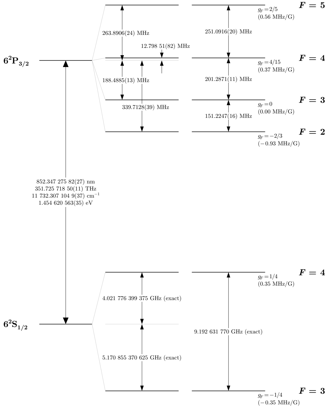
Figure 2: Cesium D_2 transition hyperfine structure, with frequency splittings between the hyperfine energy levels. The excited-state values are taken from [31], and the ground-state values are exact, as a result of the current definition of the second. The relative hyperfine shifts are shown to scale within each hyperfine manifold (but visual spacings should not be compared between manifolds or to the optical splitting). The approximate Landé g_F -factors for each level are also given, with the corresponding Zeeman splittings between adjacent magnetic sublevels.
