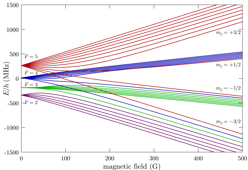
Figure 6: Cesium 6^2P_{3/2} ( D_2 excited) level hyperfine structure in an external magnetic field. The levels are grouped according to the value of F in the low-field (Zeeman) regime and m_j in the strong-field (hyperfine Paschen-Back) regime.
