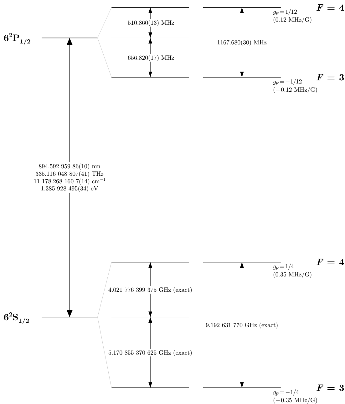
Figure 3: Cesium D 1 transition hyperfine structure, with frequency splittings between the hyperfine energy levels. The excited-state values are taken from [11, 33], and the ground-state values are exact, as a result of the current definition of the second. The relative hyperfine shifts are shown to scale within each hyperfine manifold (but visual spacings should not be compared between manifolds or to the optical splitting). The approximate Landé g_F -factors for each level are also given, with the corresponding Zeeman splittings between adjacent magnetic sublevels.
