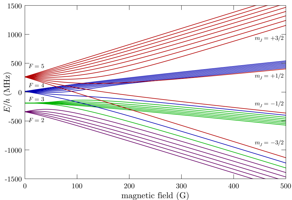
Figure 6: Cesium 6^2P_{3/2} (D 2 excited) level hyperfine structure in an external magnetic field. The levels are grouped according to the value of F in the low-field (Zeeman) regime and m_j in the strong-field (hyperfine Paschen-Back) regime.
