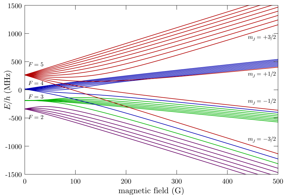
Figure 6: Cesium 6^2P_{3/2} (D 2 excited) level hyperfine structure in an external magnetic field. The levels are grouped according to the value of F in the low-field (Zeeman) regime and m_j in the strong-field (hyperfine Paschen-Back) regime.
