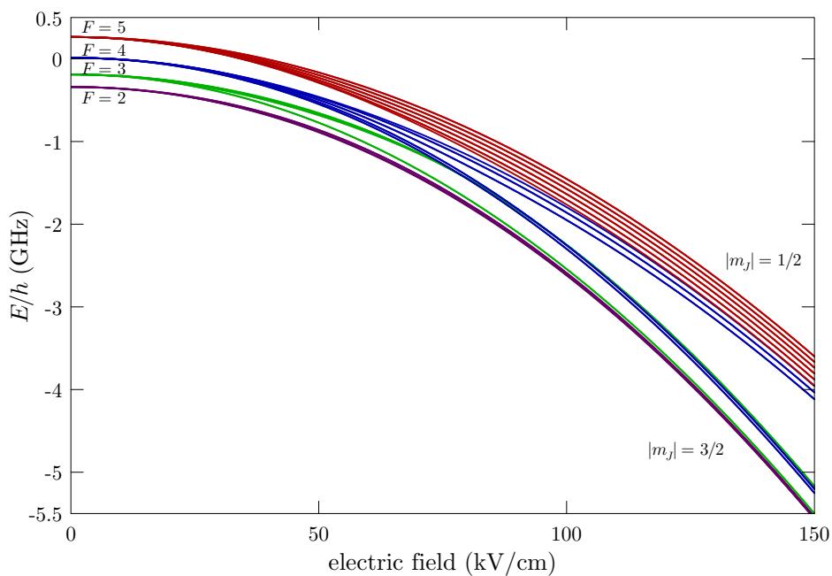
Figure 7: Cesium 6^2P_{3/2} (D 2 excited) level hyperfine structure in a constant, external electric field. The levels are grouped according to the value of F in the low-field (Zeeman) regime and |m_j| in the strong-field (“electric” hyperfine Paschen-Back) regime. Levels with the same values of F and |m_F| (for a weak field) are degenerate.
