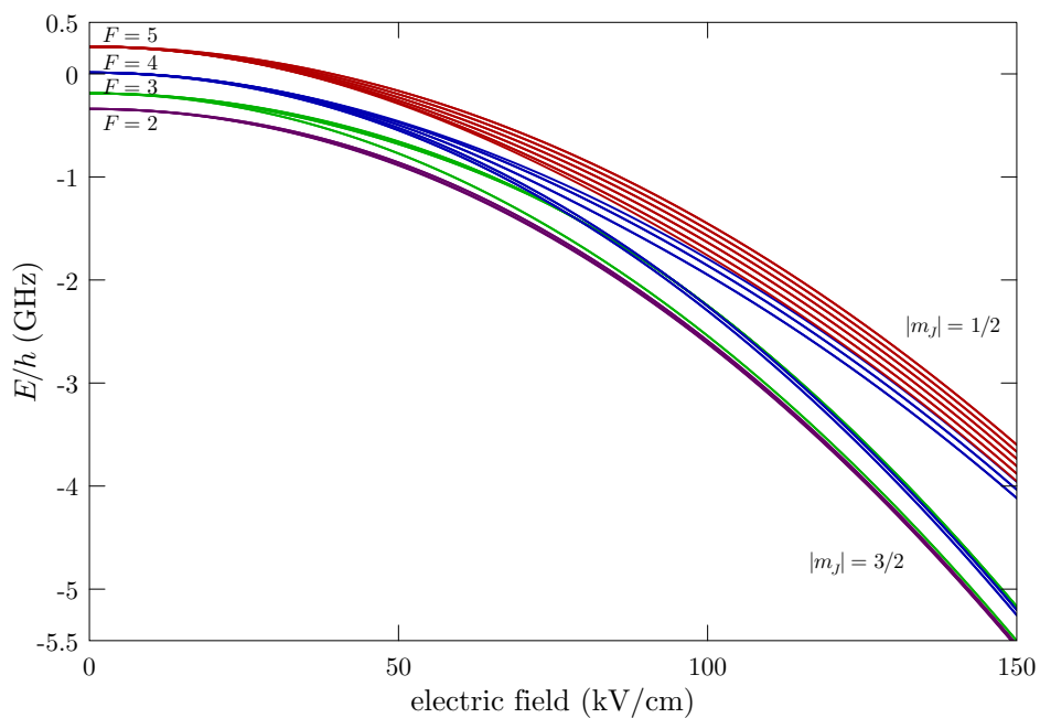
Figure 7: Cesium 6^2P_{3/2} ( D_2 excited) level hyperfine structure in a constant, external electric field. The levels are grouped according to the value of F in the low-field (Zeeman) regime and |m_j| in the strong-field ("electric" hyperfine Paschen-Back) regime. Levels with the same values of F and |m_F| (for a weak field) are degenerate.
